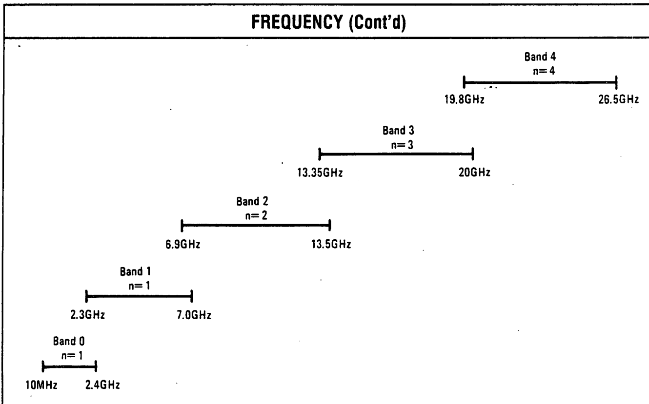
Figure 1. Frequency Ranges and Bandswitch Points in Swept Modes
