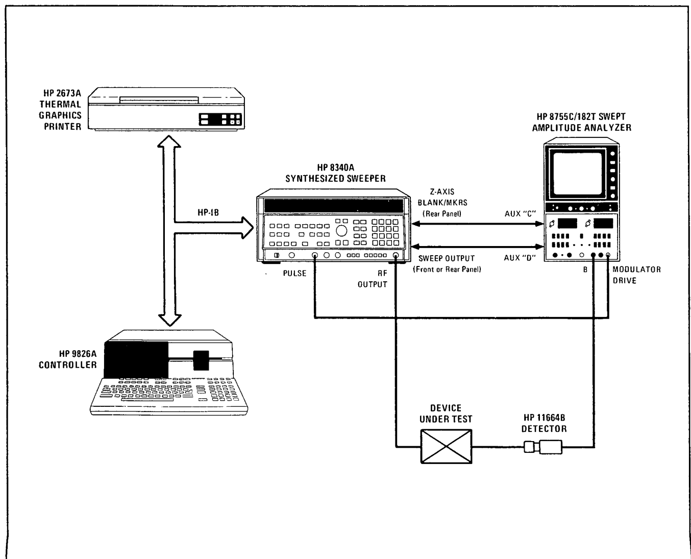
Figure 2. Equipment Setup
