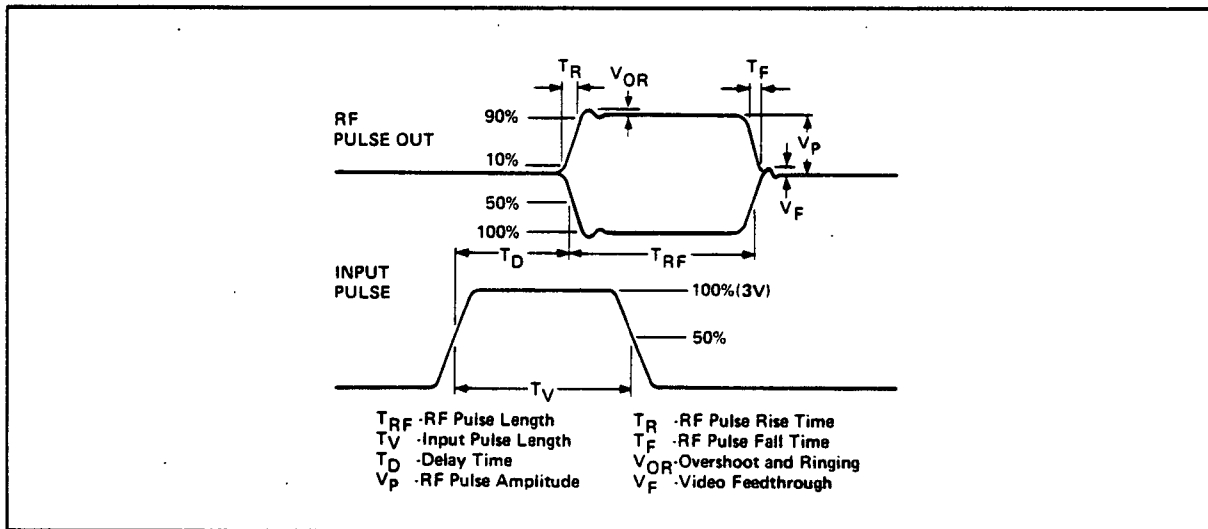
Figure 4-12. Pulse Definitions
