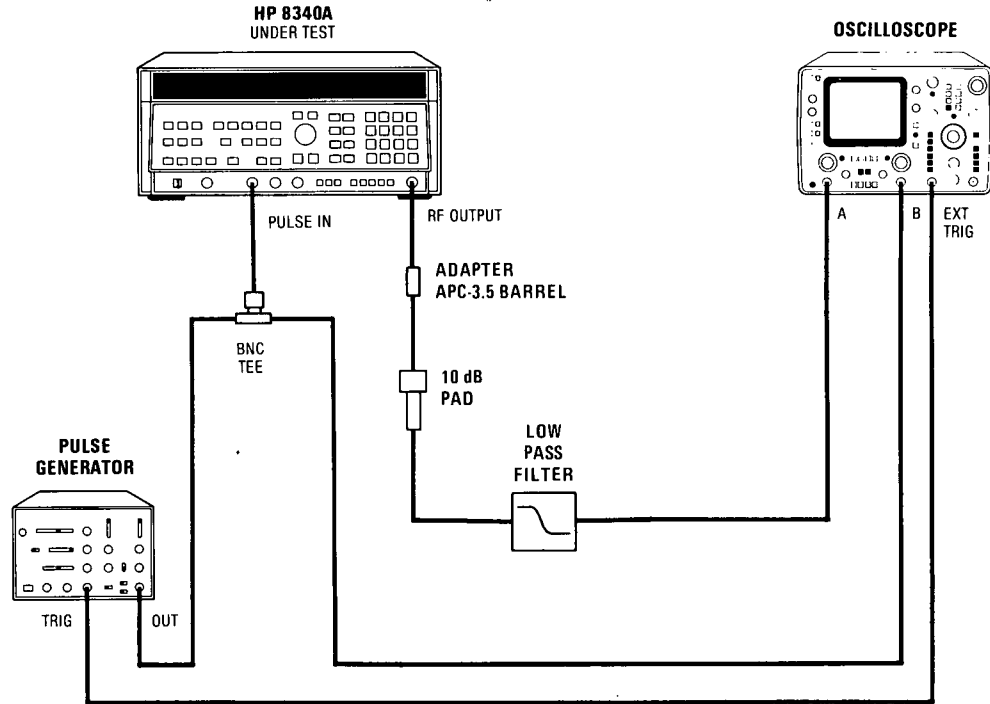
Figure 4-17. Pulse Modulation Video Feedthrough Test Setup
