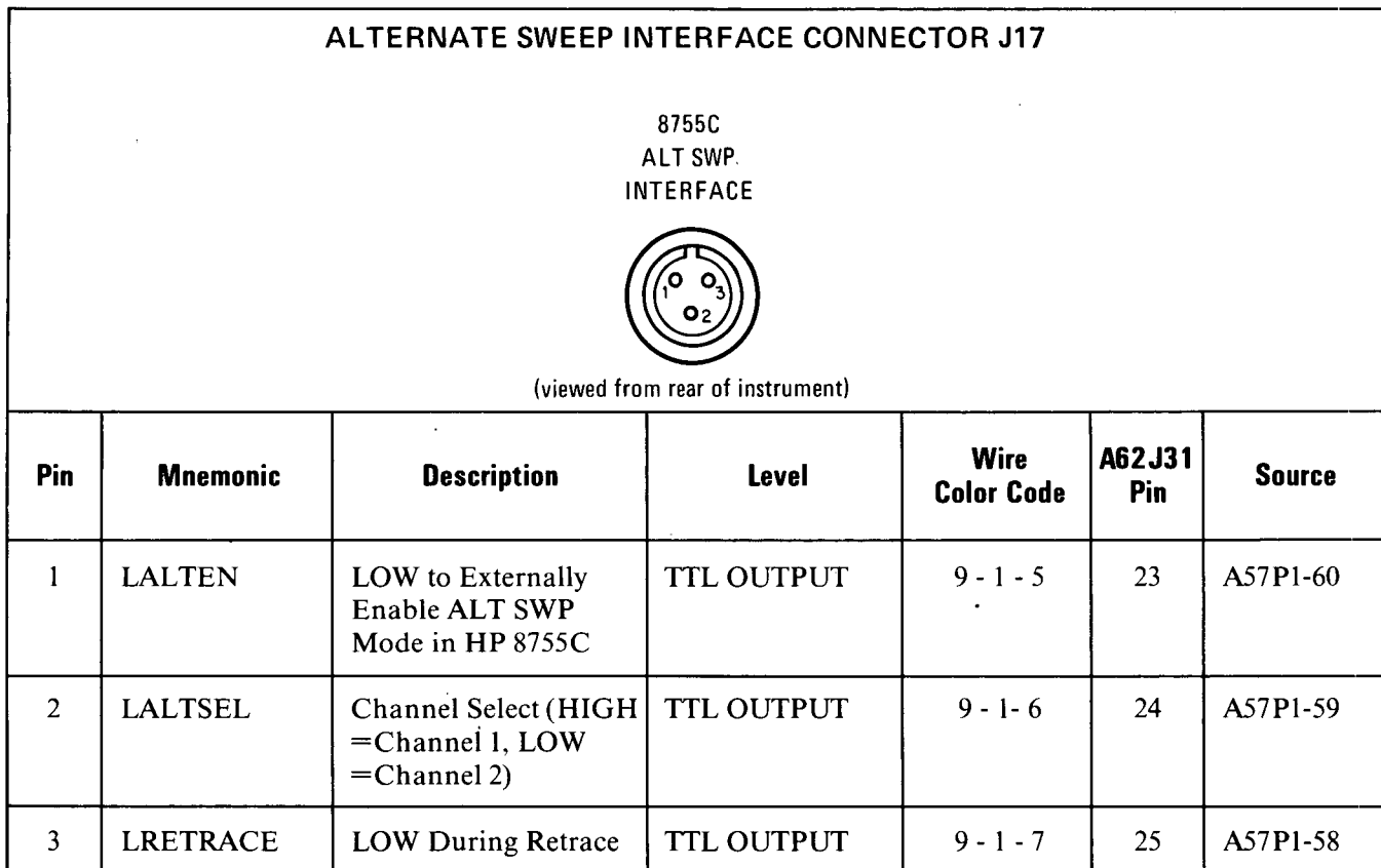
Figure 2-4. 8755C INTERFACE Connector Signal/Pin Configuration
